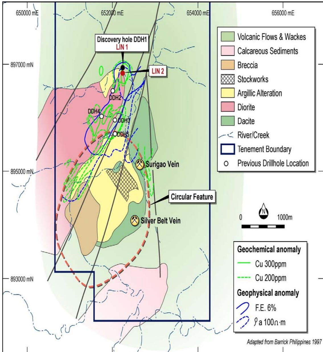
Figure 1: Geological map of the Lingig area
